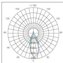
MHT8597-40W-3000K-40°
