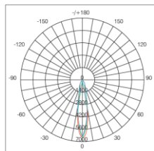
MHT8596A-20W-3000K-38°
